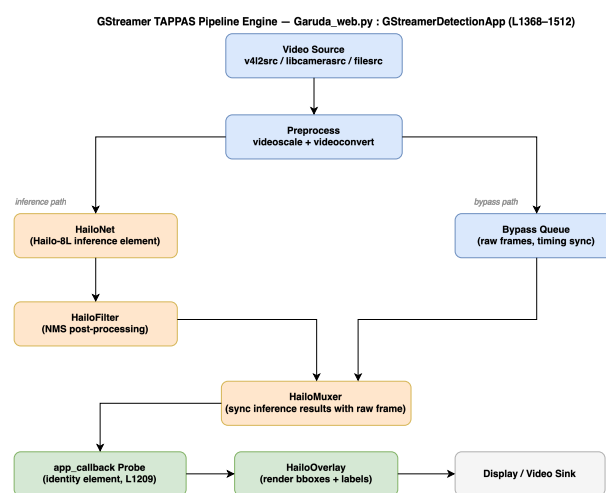
FIGURE 3. GStreamer TAPPAS pipeline: source → preprocess → (HailoNet + NMS || bypass queue) → HailoMuxer → identity callback → overlay → sink.
